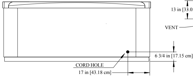
LEFT VIEW
